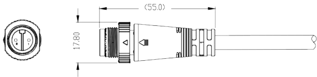
M15 male plug
