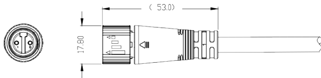
M15 female plug
